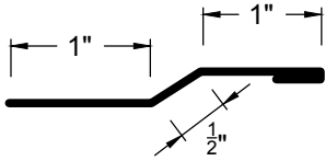
Valley Cleat VC-1
