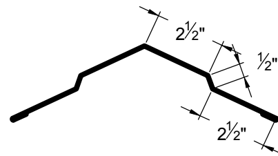
DELUXE RIDGE CAP RC-3
